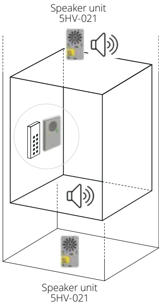
Helpy Compact - NB wall-mounted inside the elevator car
